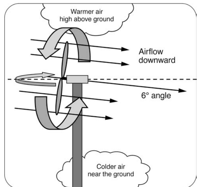
Figure 2. Wind machines pull warm air down from high above a field, blowing it downward and outward, pushing away cold air near target crops and replacing it with warmer air.
