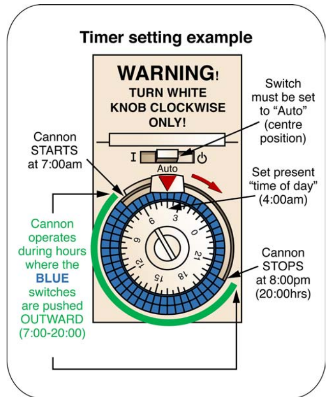
Figure 5. Inside a bird banger control system box, an operator can adjust when a bird banger starts in the morning and stops in the evening. The setting shown is appropriate for September 26 at Harrow as per Table 1.
