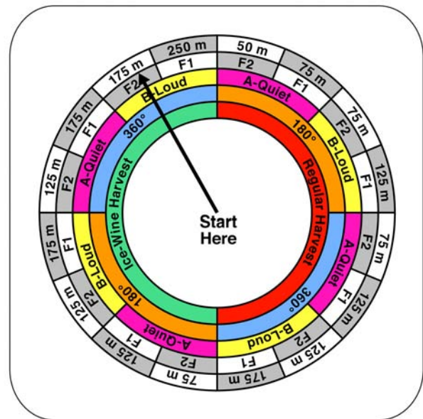
Figure 2. Ring-graph used to determine bird banger setbacks to neighbours based on management strategies.
