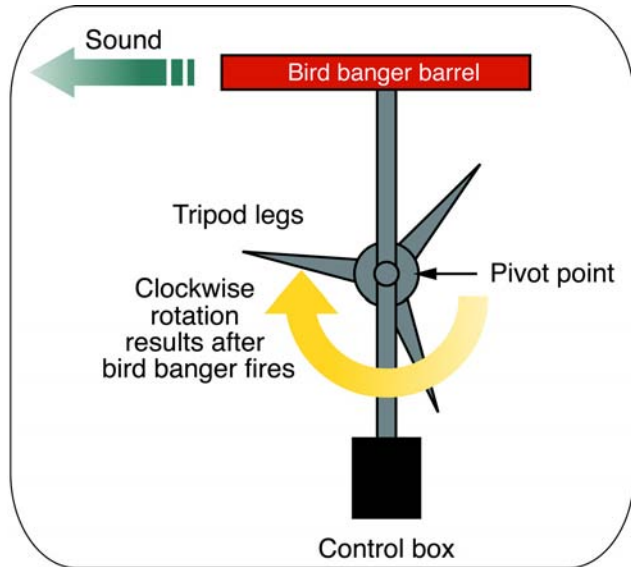
Figure 4. This overhead view shows as sound waves exit a bird banger barrel it causes recoil, turning it clockwise. Tests show it can spin up to 10 times before stopping.
